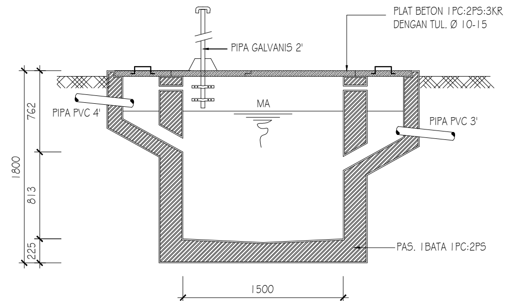
DETAIL POTONGAN - A 1:50
