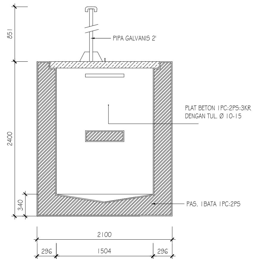
DETAIL POTONGAN - B 1:50
